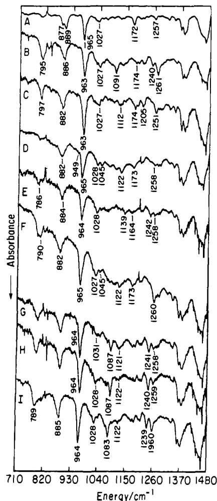
Figure 5. The infrared spectra of (A) 12-ethyl,13- cis Schiff base, (B) 12- N -ethano Schiff base and its (C) 14D, (D) 15D, (E) 14,15- ^{13}\text{C} , 15D, (F) 14,15D 2 , (G) 14- ^{13}\text{C} , (H) 15- ^{13}\text{C} , and (I) 14,15- ^{13}\text{C} derivatives. Infrared spectra were obtained from a thin film on a KBr window.
