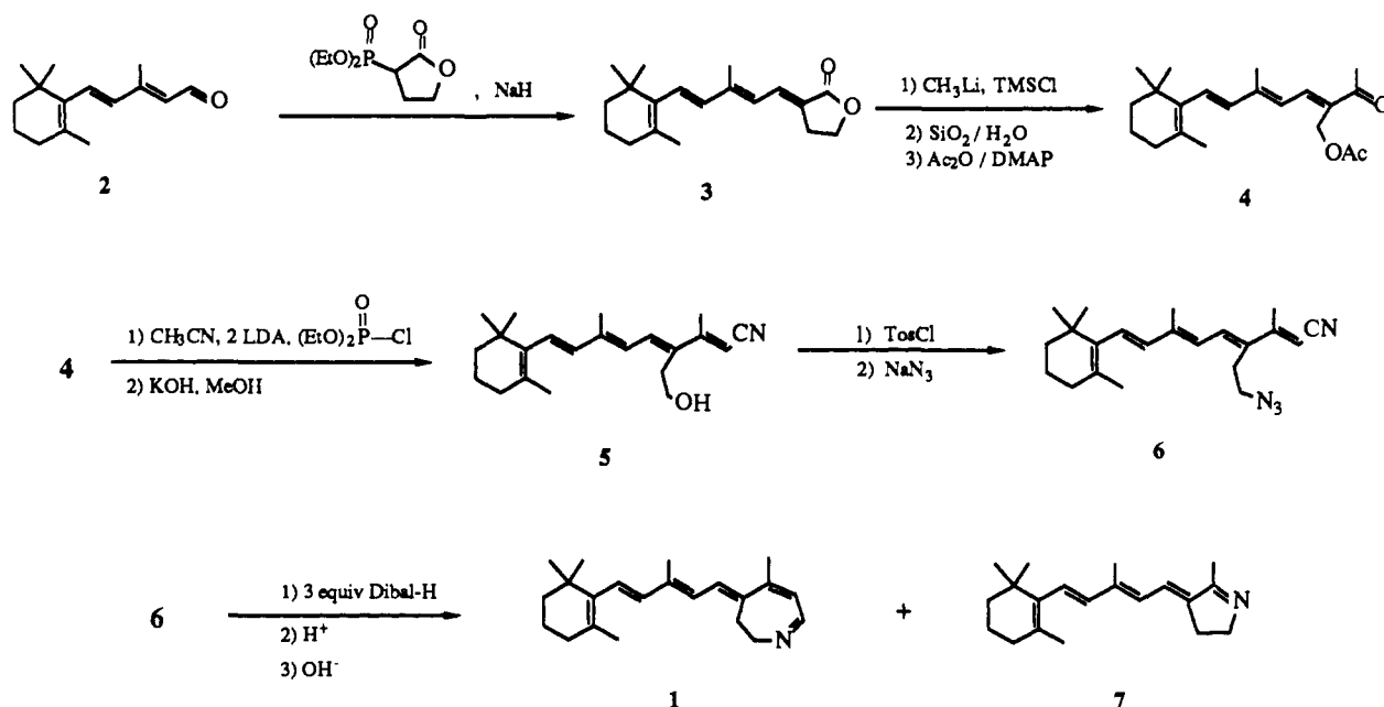
Scheme I. Synthesis of the 12- N -Ethano-retinal Schiff Base 1
