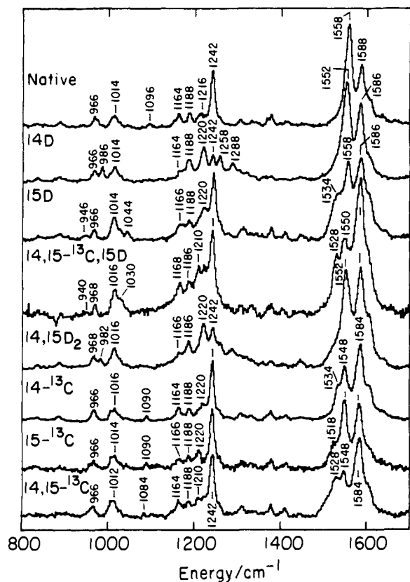
Figure 4. Raman spectra of the 12- N -ethano retinal Schiff base and its 14D, 15D, 14,15- ^{13}\text{C} , 15D, 14,15D 2 , 14- ^{13}\text{C} , 15- ^{13}\text{C} , and 14,15- ^{13}\text{C} derivatives. All Raman spectra were obtained using a stationary chloroform solution with 25–50 mW of spherically focused 752.4-nm excitation.
